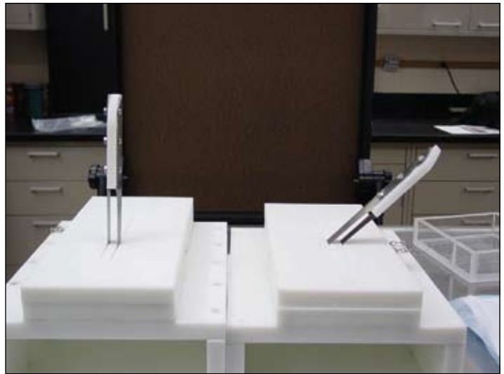
90° and 45° slice boxes
