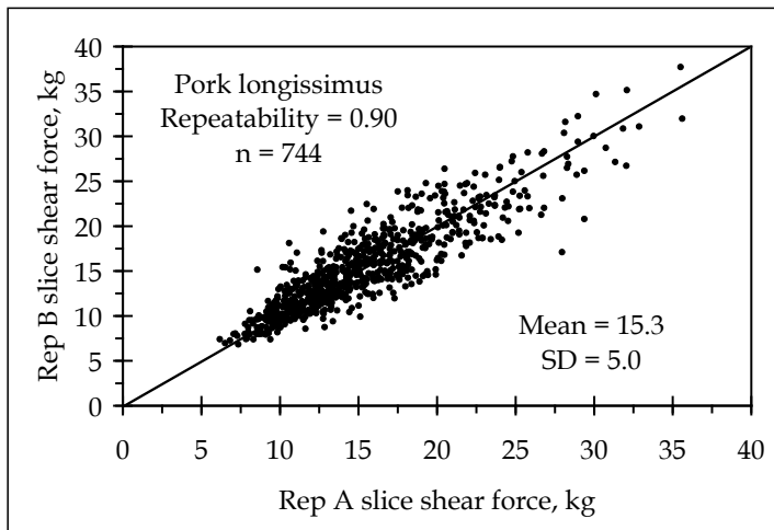
Figure 3. Repeatability of slice shear force for pork and lamb longissimus (From Shackelford et al., 2004ab)
