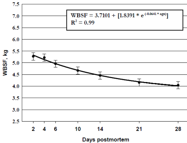
Figure 12. Least squares means \pm standard error of the mean of Warner-Bratzler shear force (WBSF) for Select rectus femoris at 7 postmortem aging periods, and the non-linear regression model fit to these points. The variable “age” is the days of postmortem aging. The R^2 is the maximum proportion of total variability explained by the model. The constant “e” equals the base of the natural logarithm (2.718282).
